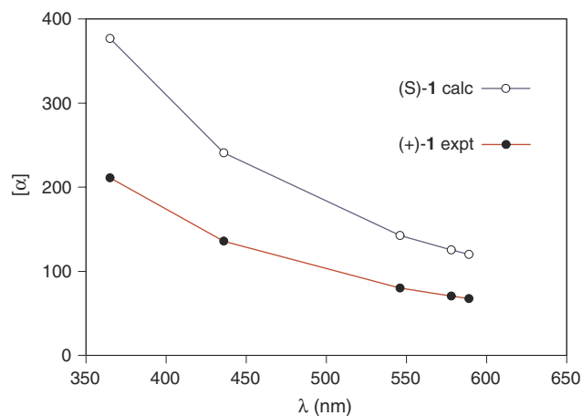
Fig. 7 B3LYP/aug-cc-pVDZ//B3LYP/6-31G* [\alpha] values for S-1 and experimental [\alpha] values for (+)- 1
