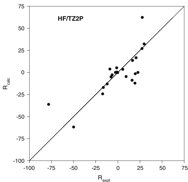
Fig. 8 Comparison of the HF/TZ2P and experimental rotational strengths. The straight line , of slope +1, is the “line of perfect agreement”
