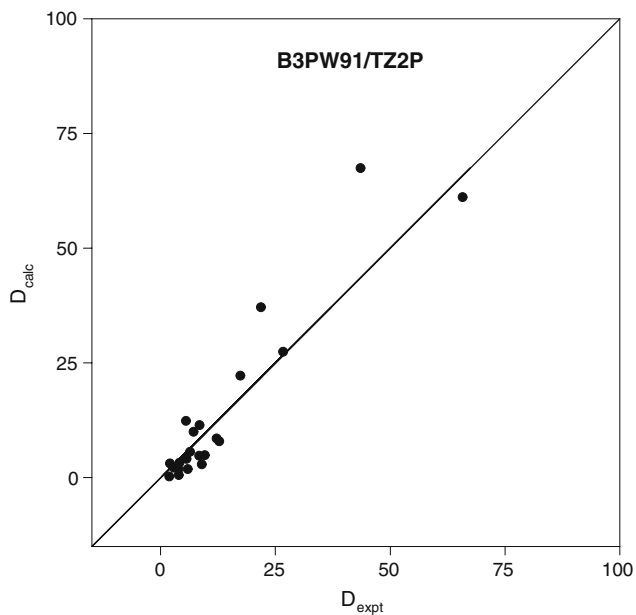
Fig. 5 Comparison of the B3PW91/TZ2P and experimental dipole strengths. For bands assigned to multiple vibrational modes, calculated dipole strengths are the sums of the dipole strengths of contributing modes. The straight line , of slope +1, is the “line of perfect agreement”
