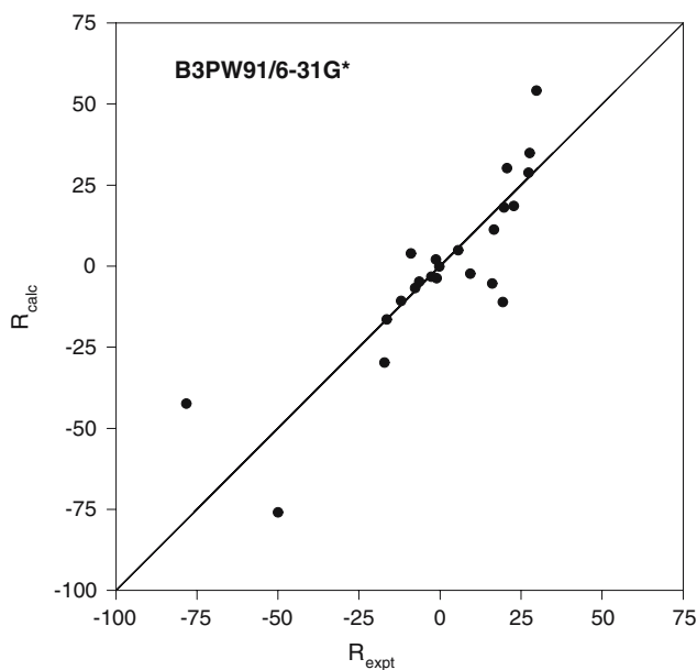
Fig. 9 Comparison of the B3PW91/6-31G* and experimental rotational strengths. The straight line , of slope +1, is the “line of perfect agreement”
