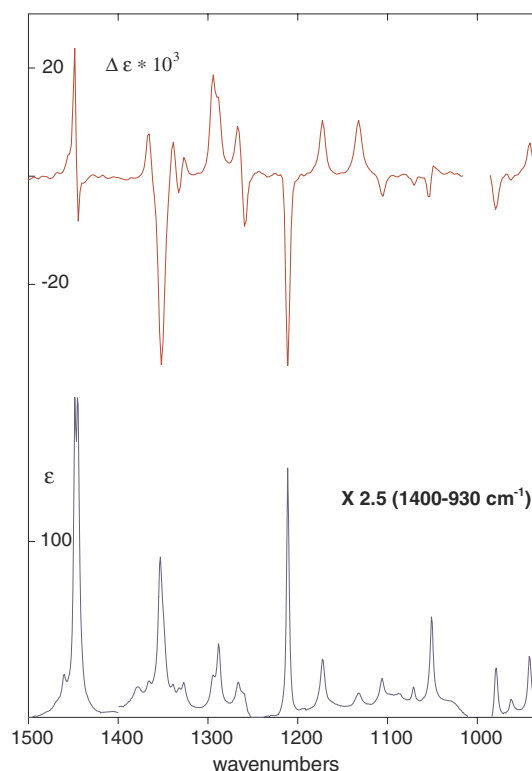
Fig. 1 The experimental IR and VCD spectra of (+)- 1 in CCl 4 solution (0.0765 M). The VCD spectrum is normalized to 100% ee
