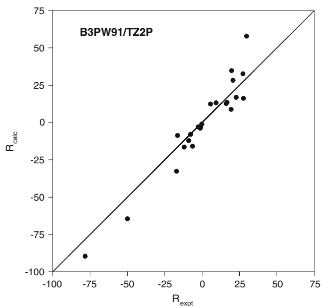
Fig. 6 Comparison of the B3PW91/TZ2P and experimental rotational strengths. For bands assigned to multiple vibrational modes, calculated rotational strengths are the sums of the rotational strengths of contributing modes. The straight line , of slope +1, is the “line of perfect agreement”
