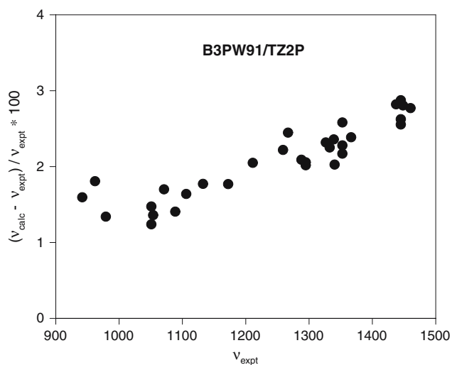
Fig. 4 Comparison of the B3PW91/TZ2P and experimental frequencies. For bands assigned to multiple vibrational modes, all calculated frequencies are compared to the corresponding experimental frequencies
